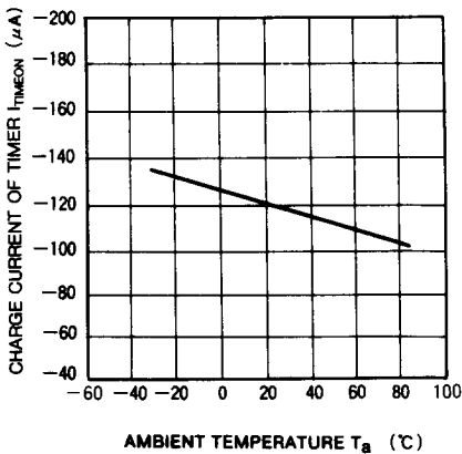
CHARGE CURRENT OF TIMER VS. AMBIENT TEMPERATURE
