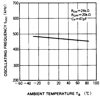
OSCILLATING FREQUENCY VS. AMBIENT TEMPERATURE
