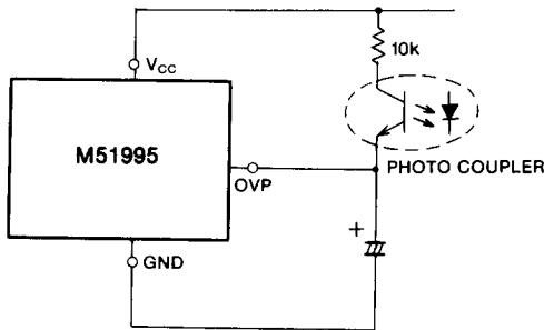
Fig. 28 Peripheral circuit of OVP terminal
