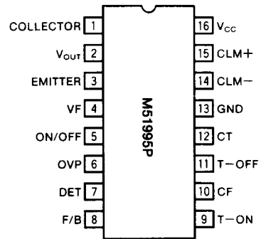
Outline 16P4
