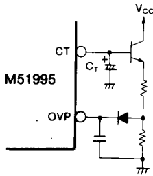
Fig. 39 Application circuit diagram to keep the non-operating condition when over load current condition will continue for specified duration
