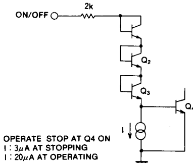
Fig. 19 ON/OFF circuit
