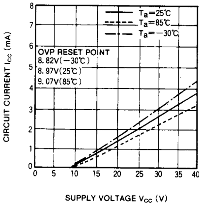
Fig. 23 CIRCUIT CURRENT VS SUPPLY VOLTAGE (OVP OPERATION)
