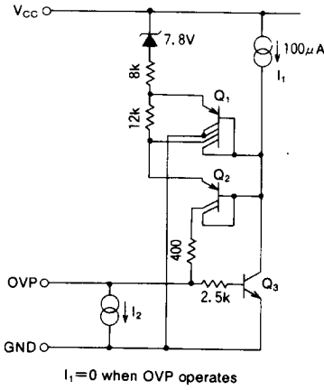
Fig. 22 Detail diagram of OVP circuit
