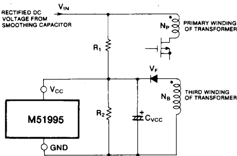
Fig. 25 Start-up circuit diagram when it is necessary to set the start and stop input voltage
